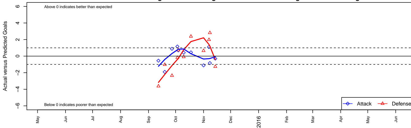
ISC Gunners Rec Spartans B99 Dots are actual minus expected GF (blue circles) and GA (red triangles). Blue line is smoothed change in attack strength. Red is smoothed change in defense strength.
